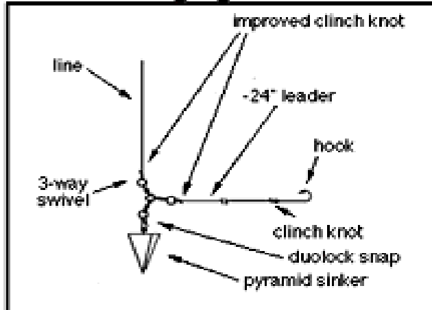
Surf fishing rig for red drum
