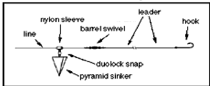
Surf fishing rig for red drum
